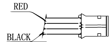
JST PHR-2 HOUSING BACK VIEW S=2
